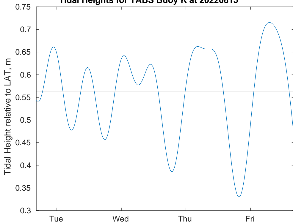
Tidal Heights for TABS Buoy K at 20220815
